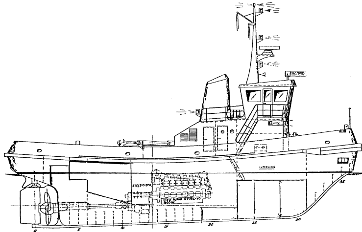
Tug M/V "STEVNS GUARD" Built by Asi-Verken AAmal Sweden 1977. Call sign OWLE. IMO No. 7418335 GSM +45
